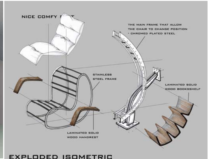
EXPLODED ISOMETRIC
